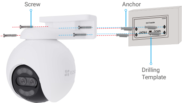
Fig. 2 Wall Mount
